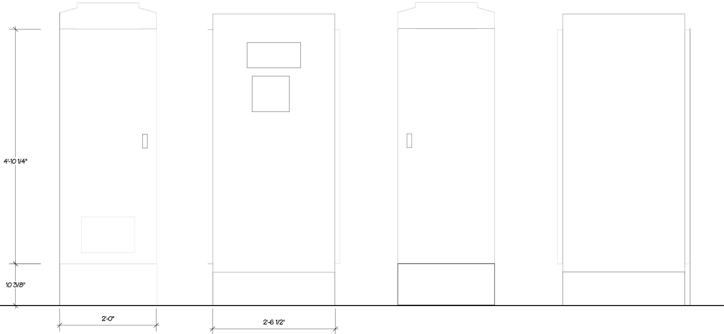
Shaker Arts Council Utility Box Template Scale: 1" = 1'-0"
